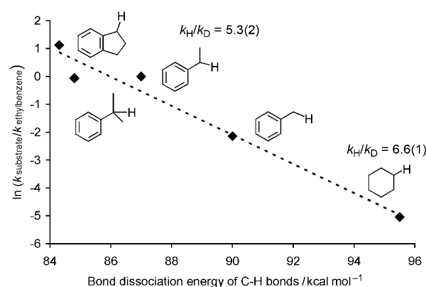
Figure 1. Catalytic rates of amination at 110 °C relative to ethylbenzene [ \ln(k_{\text{substrate}}/k_{\text{ethylbenzene}}) ] versus C–H bond strength. All rates were normalized for the number of equivalent participating C–H bonds.
